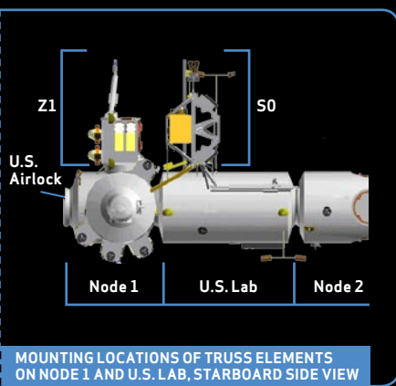
VIEW OF TOP/FORWARD/STARBOARD
